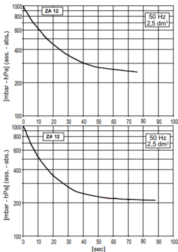
NOTE: Curves refers to 1013mbar (abs.) pression and 20°C temp. (tolerance ±10%).
